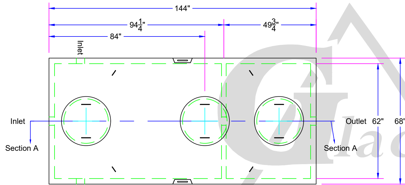
Top View
