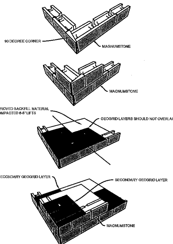
OUTSIDE CORNER
