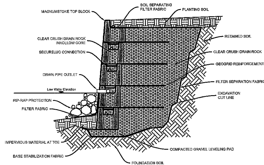
WATER APPLICATION
