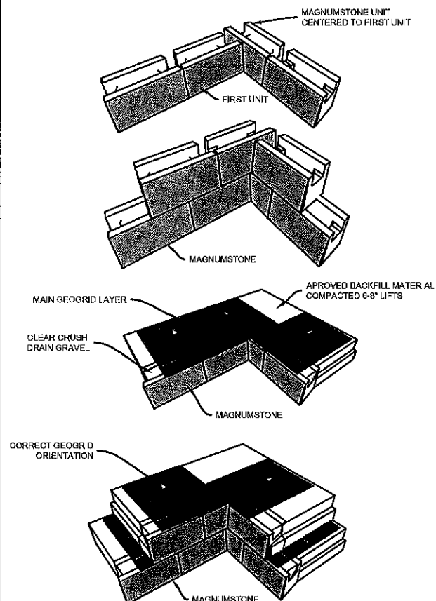
INSIDE CORNER
