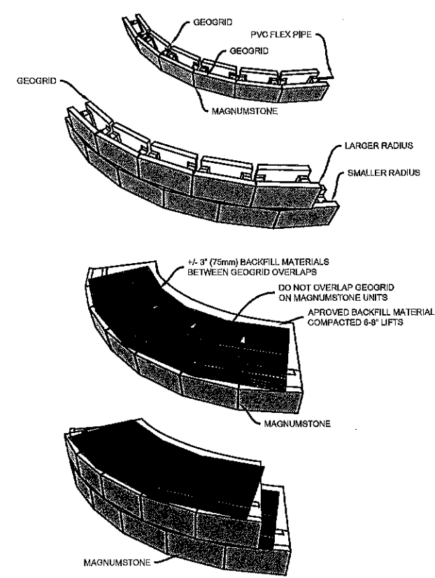
OUTSIDE CURVE
