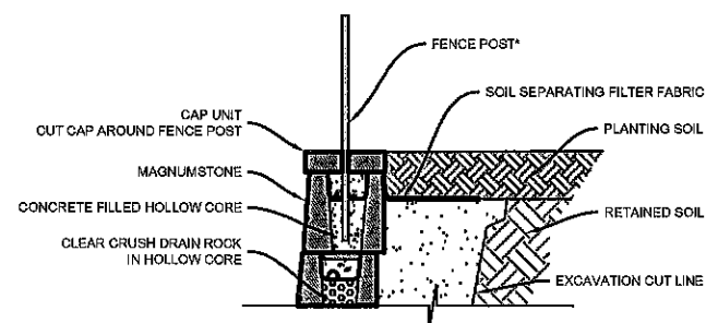
FENCE THROUGH HOLLOW CORE W /CAP
