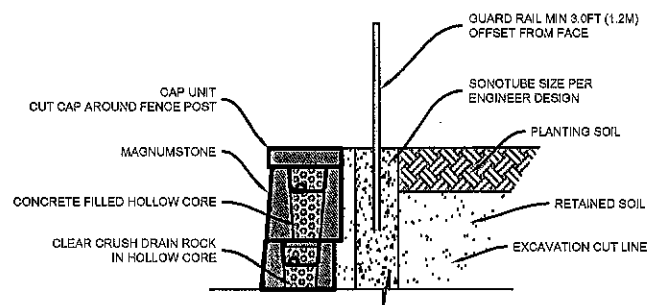
GUARD RAIL
