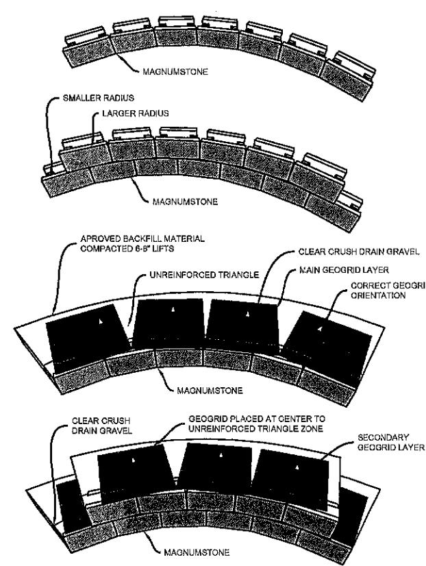
INSIDE CURVE
