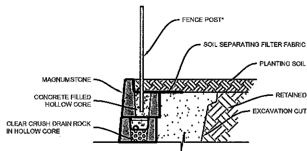
FENCE THROUGH HOLLOW CORE
