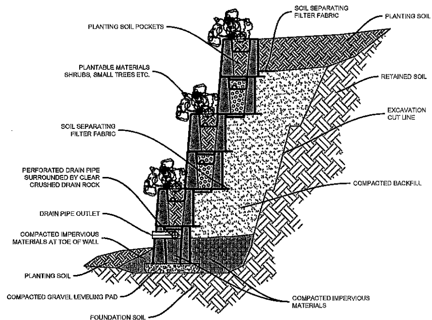
4.0 FT PLANTABLE WALL
