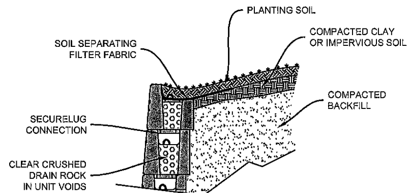
CLAY / IMPERVIOUS SWALE
