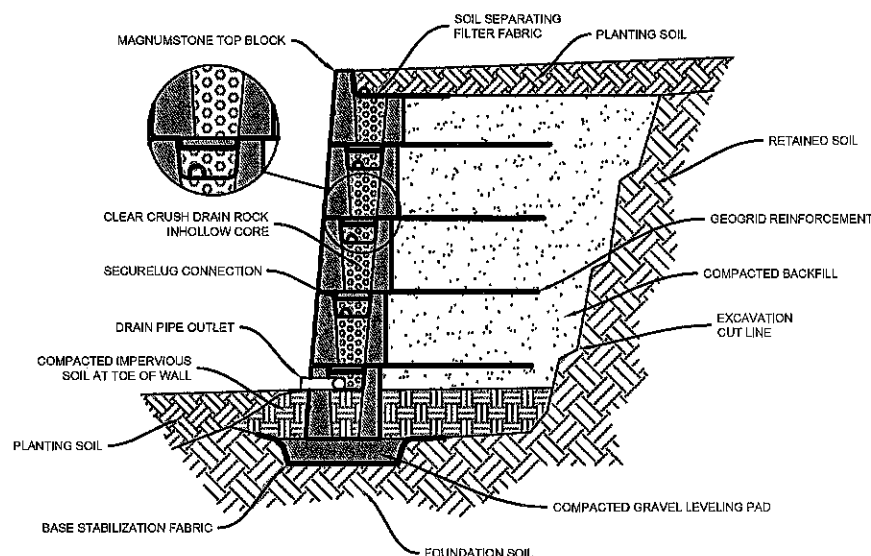
GEOGRID REINFORCED WALL
