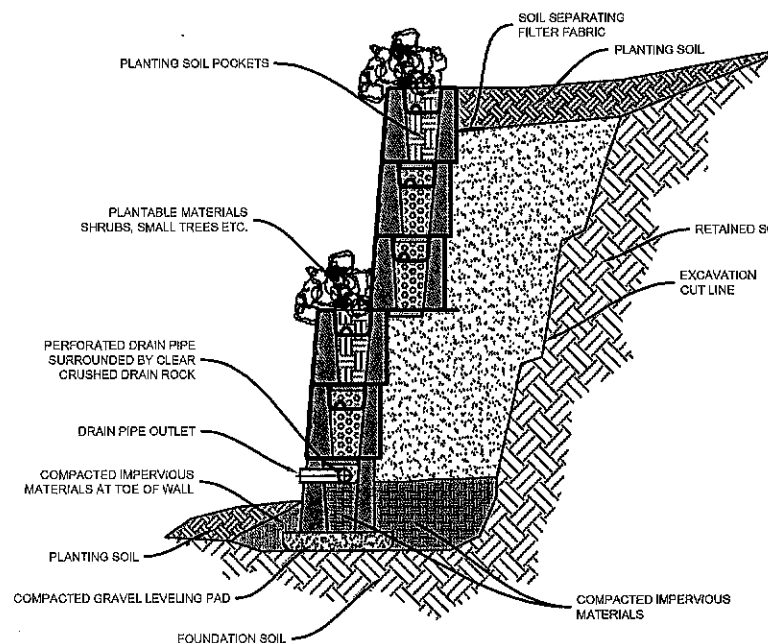
6.0 FT PLANTABLE WALL
