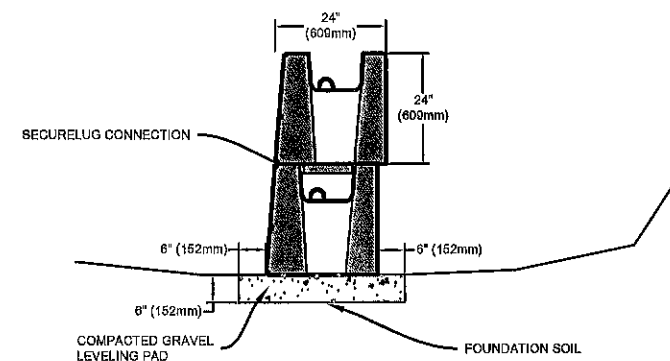
LEVELING PAD
