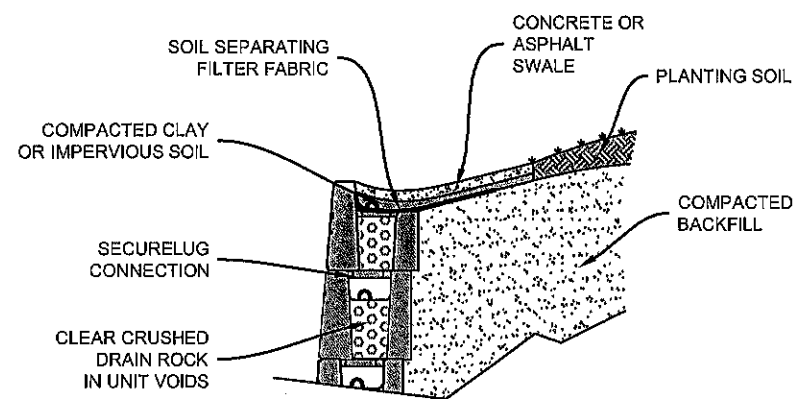
CONCRETE / ASPHALT SWALE
