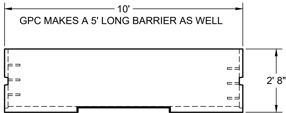
ELEVATION VIEW - FRONT
