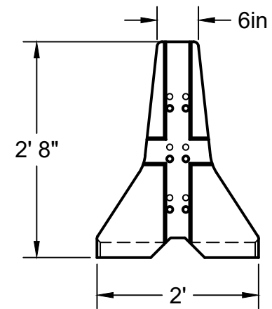
ELEVATION VIEW - SIDE
