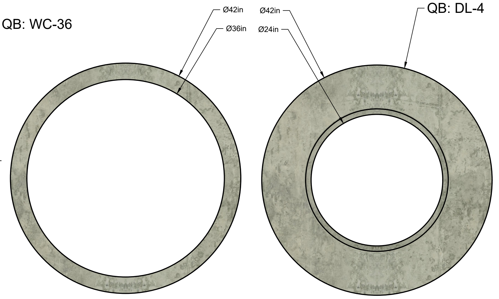
BARREL SECTIONS
